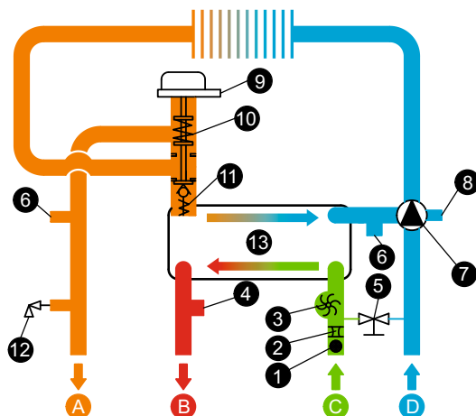
Hydraulic Circuit
