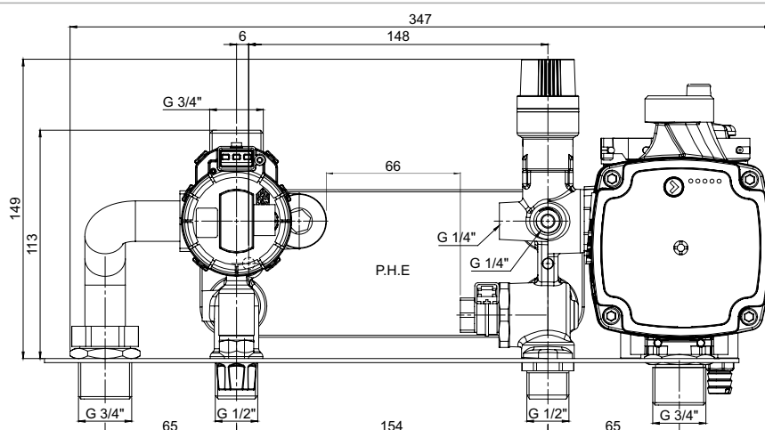
Dimensions (mm)
