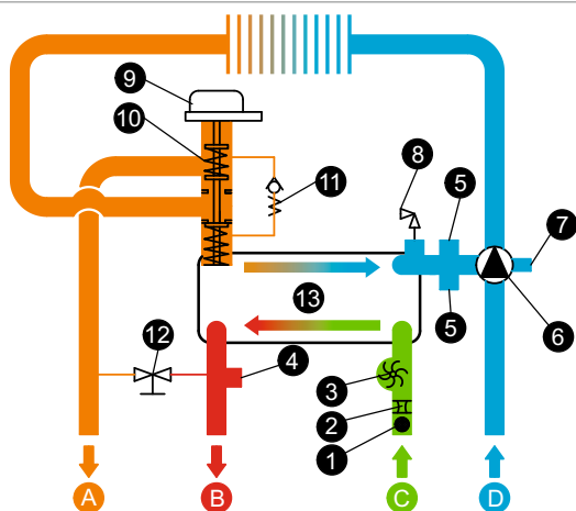
Hydraulic Circuit
