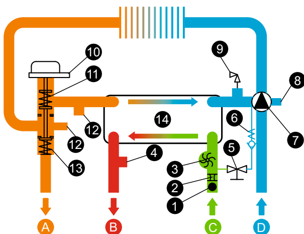
Hydraulic Circuit
