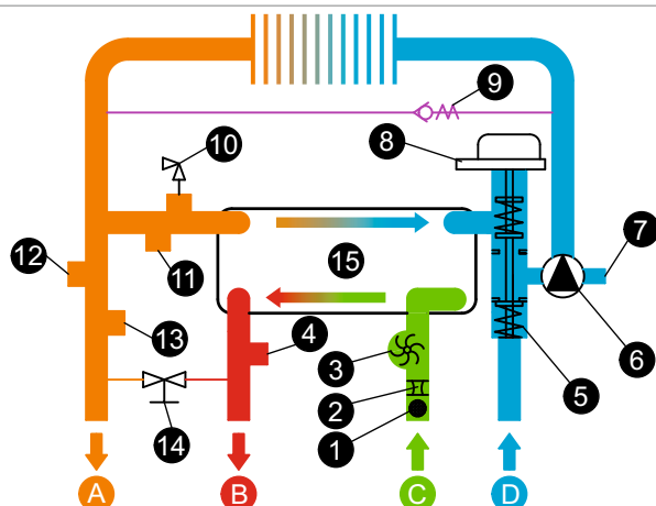
Hydraulic Circuit
