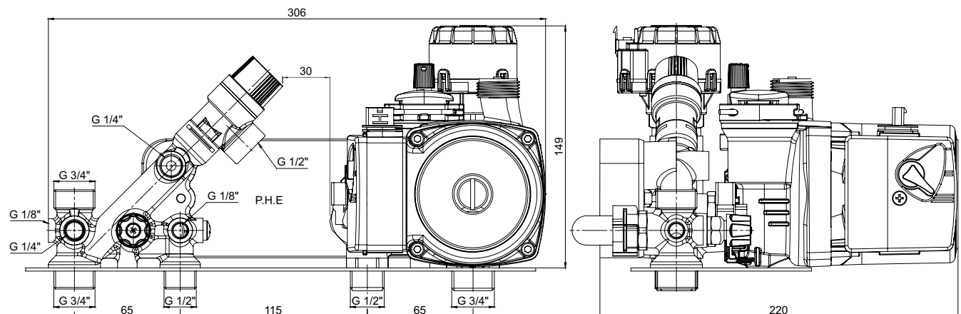
Dimensions (mm)
