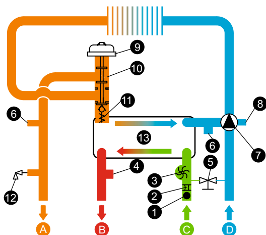
Hydraulic Circuit
