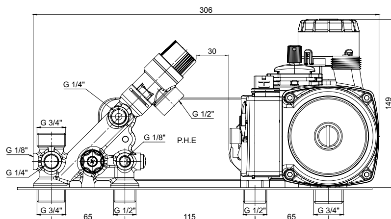
Dimensions (mm)
