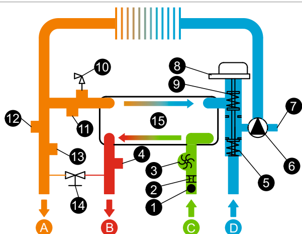
Hydraulic Circuit
