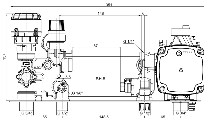
Dimensions (mm)
