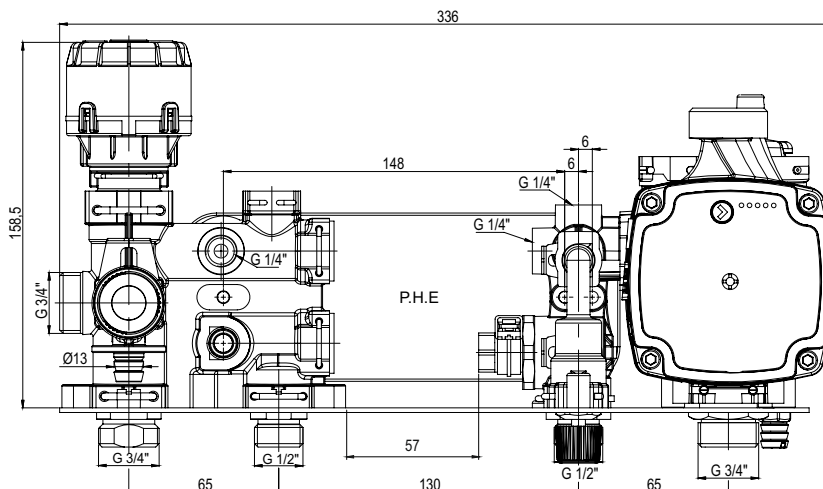
Dimensions (mm)
