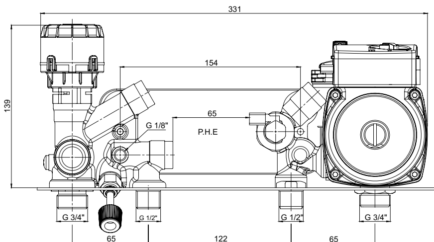
Dimensions (mm)
