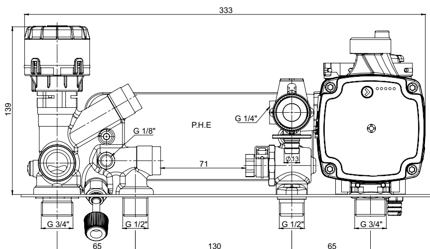
Dimensions (mm)
