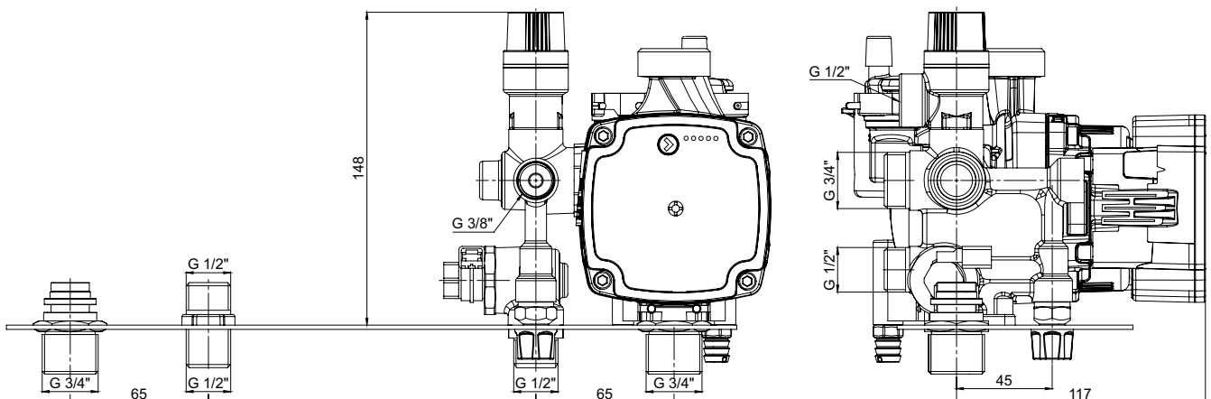
Dimensions (mm)
