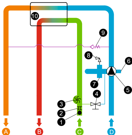
Hydraulic Circuit
