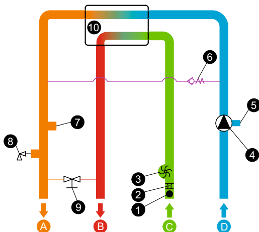
Hydraulic Circuit
