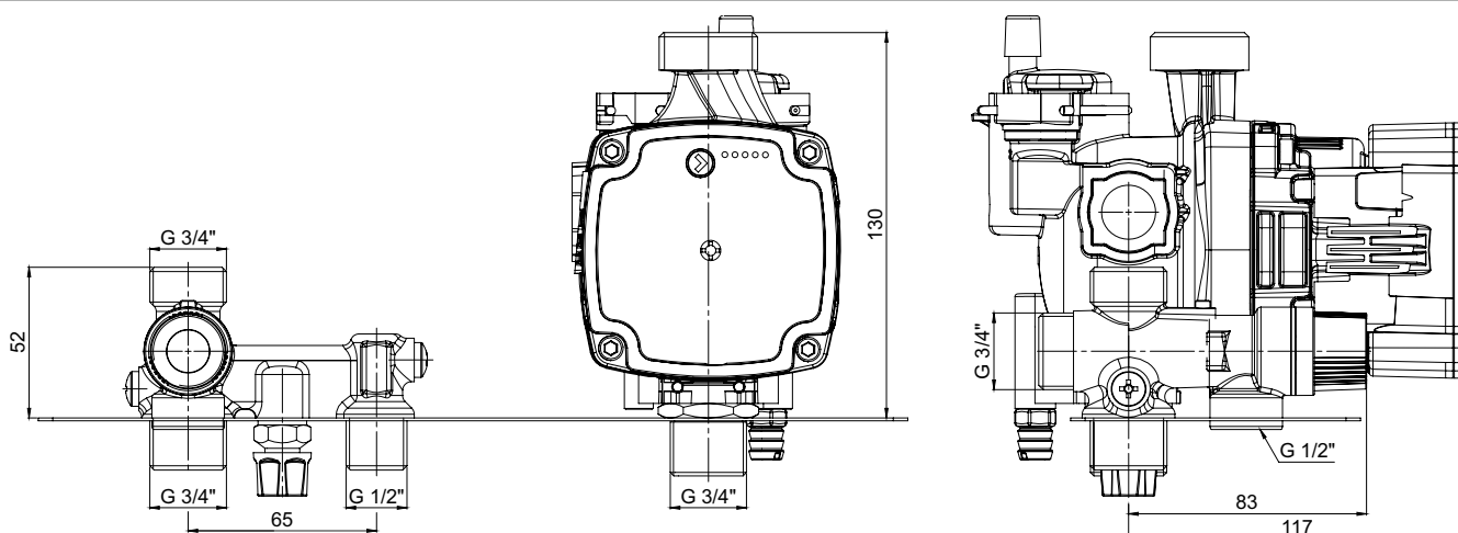
Dimensions (mm)
