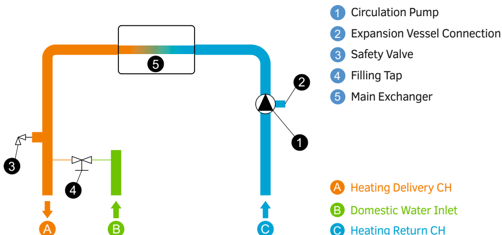
Hydraulic Circuit
