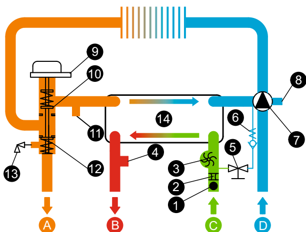
Hydraulic Circuit
