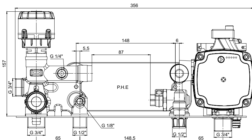
Dimensions (mm)
