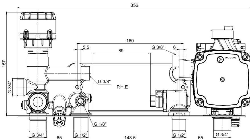
Dimensions (mm)
