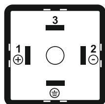
CONNECTION-PIN
